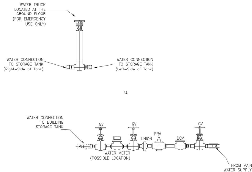
Diagram 5.1B– Incoming Mains Water Valve Detail at High Level Ground Floor or Basement (Water Meter Shown)
