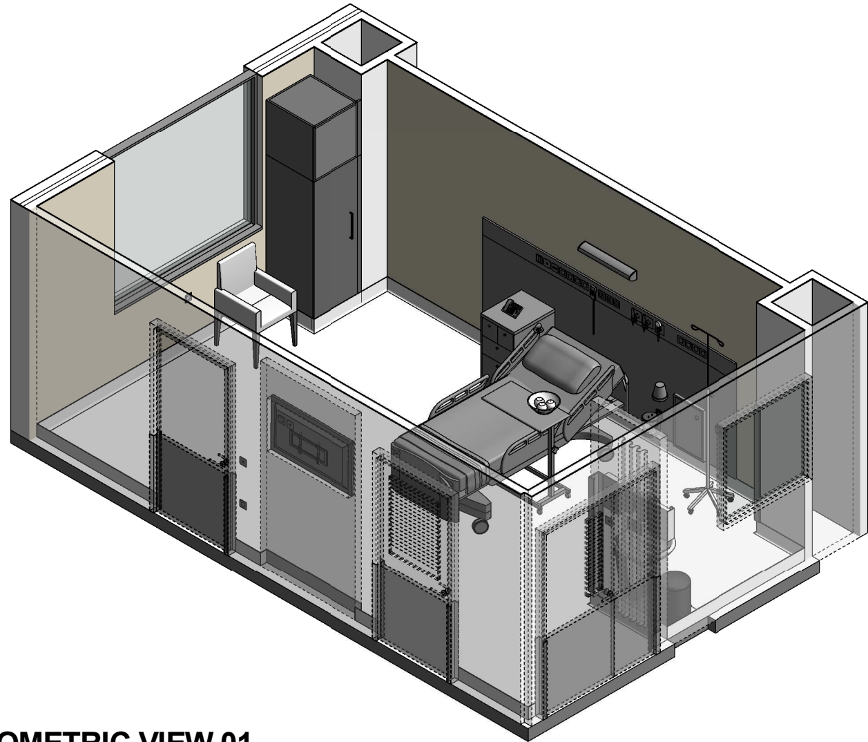
ISOMETRIC VIEW 01
