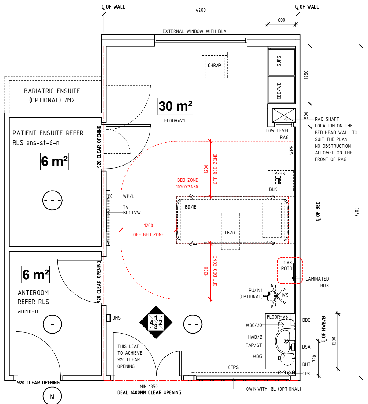
PLAN
