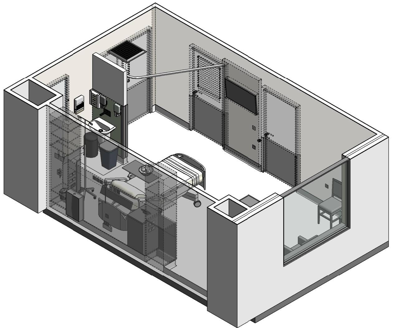
ISOMETRIC VIEW 02
