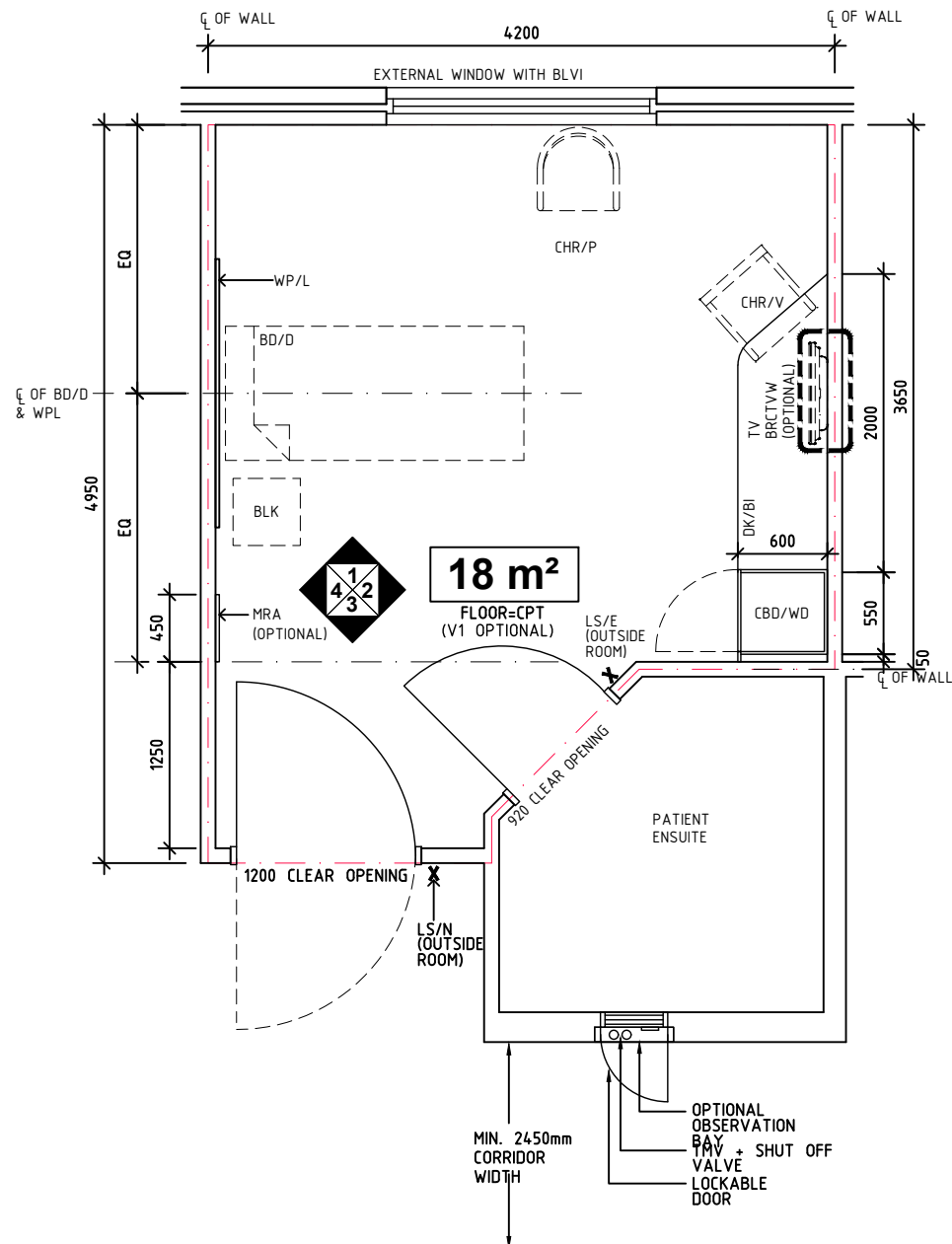
PLAN
