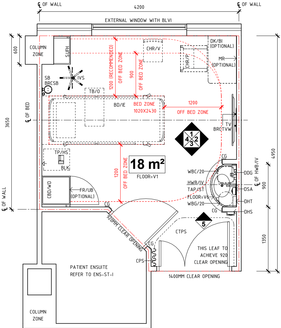
PLAN
