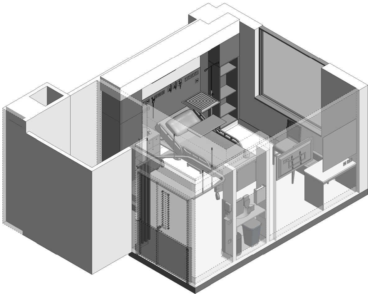
ISOMETRIC VIEW 01
