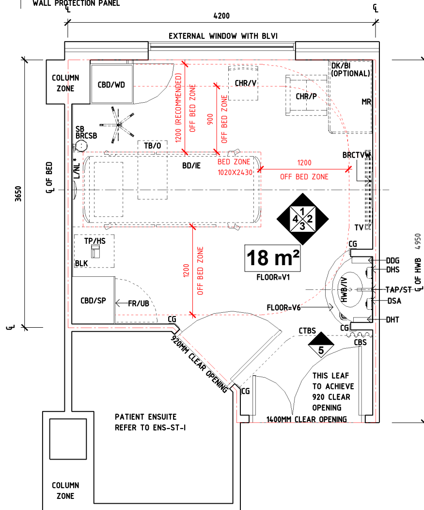
PLAN
