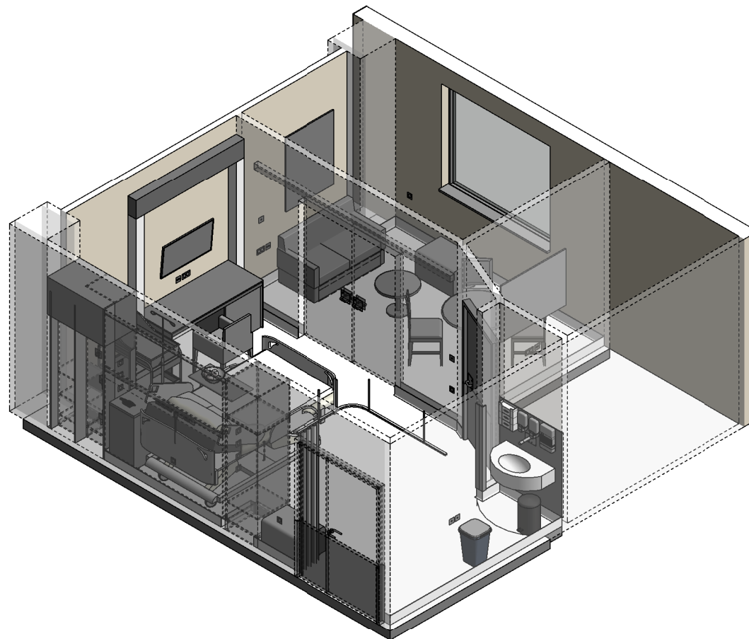
ISOMETRIC VIEW 02
