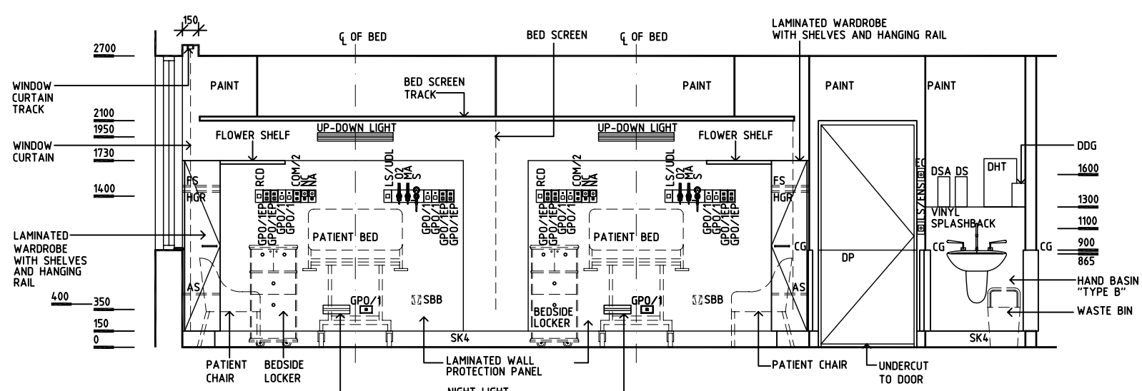
ELEVATION 2 ELEVATION 4 (MIRROR & SIMILAR)
