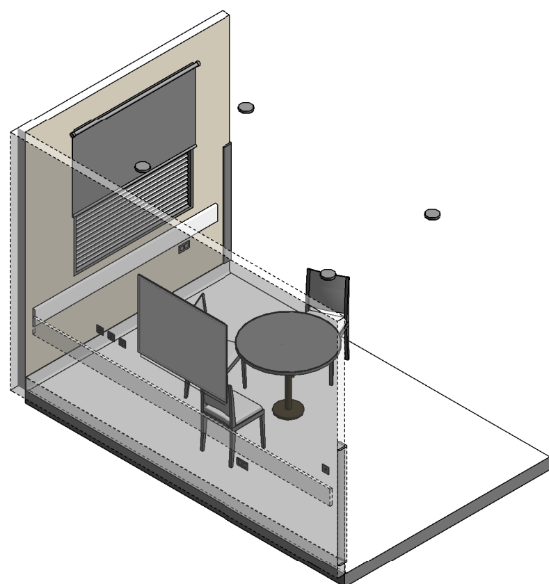
ISOMETRIC VIEW 01
