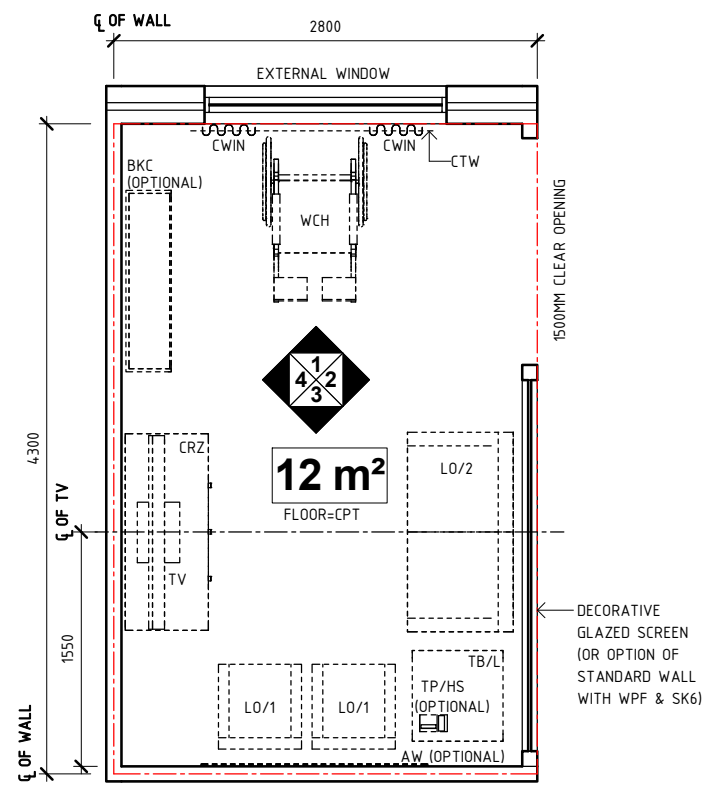
PLAN
