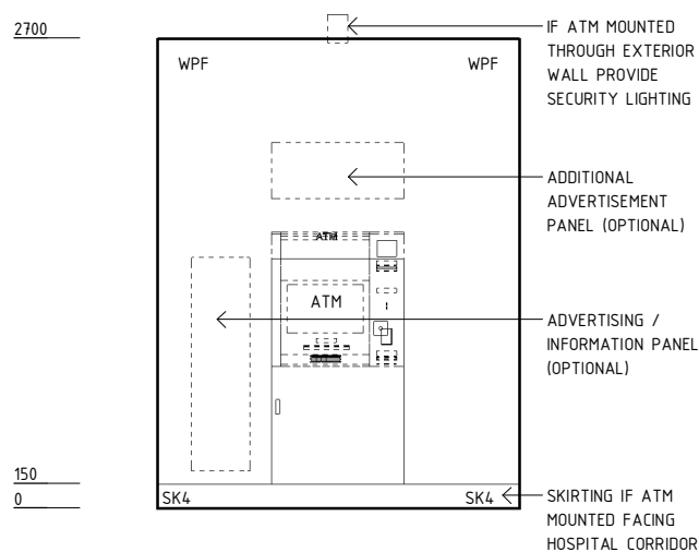
ELEVATION 03
