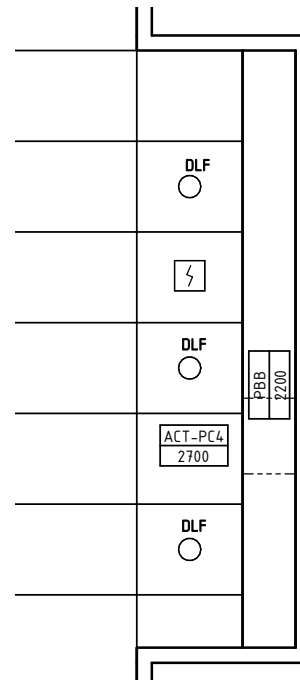
REFLECTED CEILING PLAN
