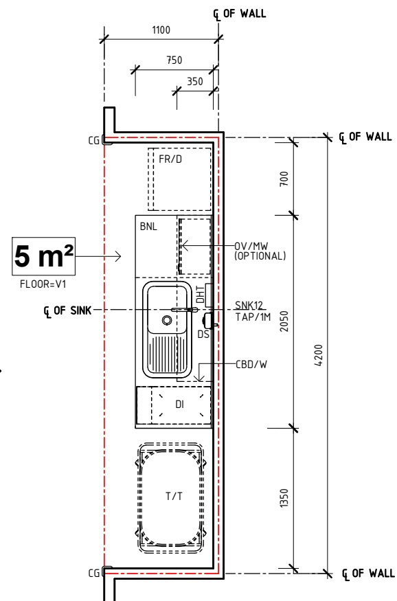
PLAN
