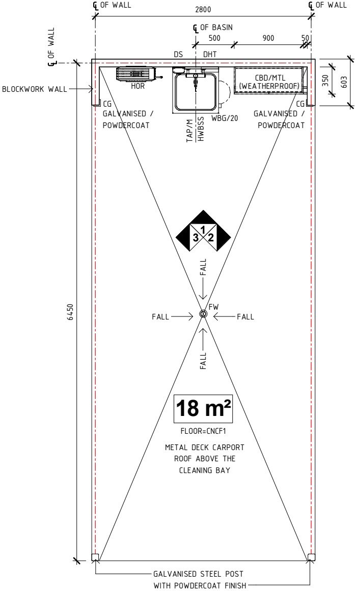
PLAN
