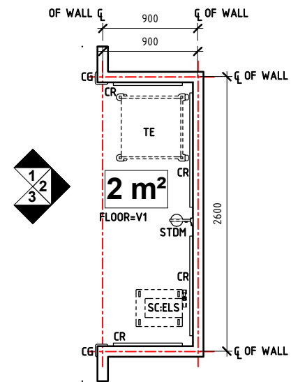
PLAN
