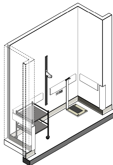
ISOMETRIC VIEW 01
