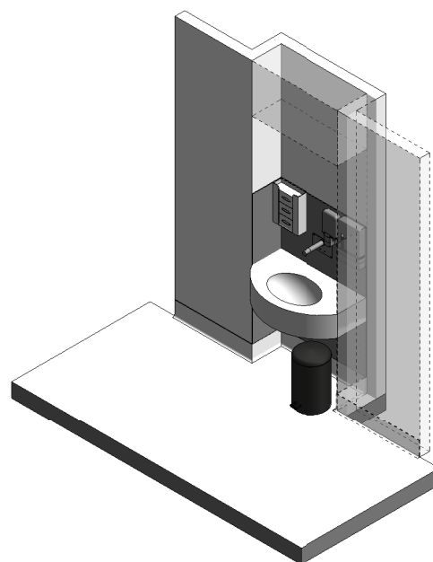
ISOMETRIC VIEW
