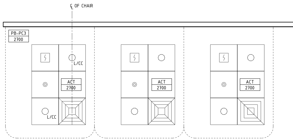
REFLECTED CEILING PLAN
