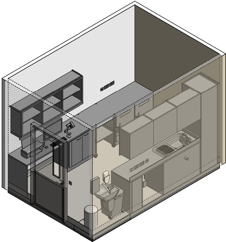
ISOMETRIC VIEW 01
