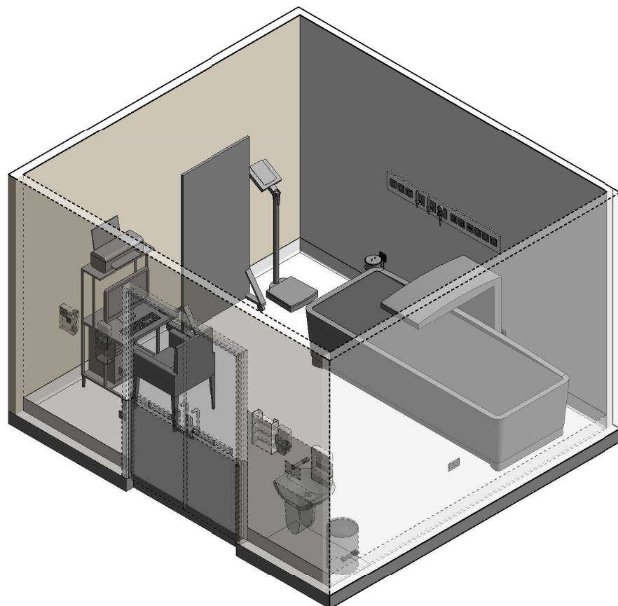
ISOMETRIC VIEW 1
