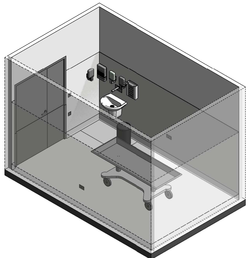
ISOMETRIC VIEW 2
