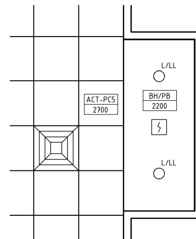
REFLECTED CEILING PLAN
