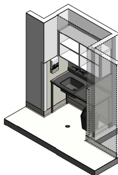
ISOMETRIC VIEW
