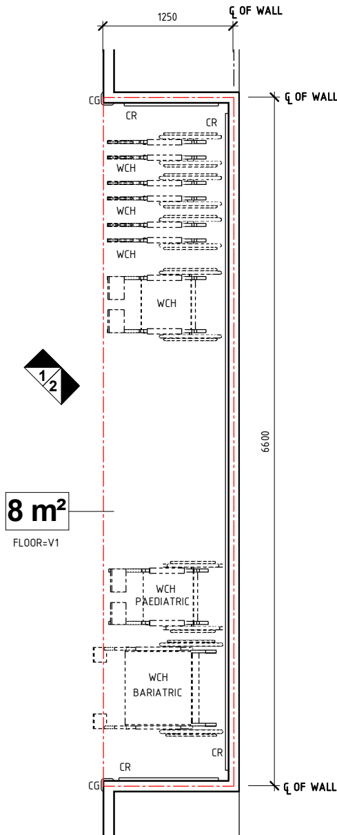
PLAN
