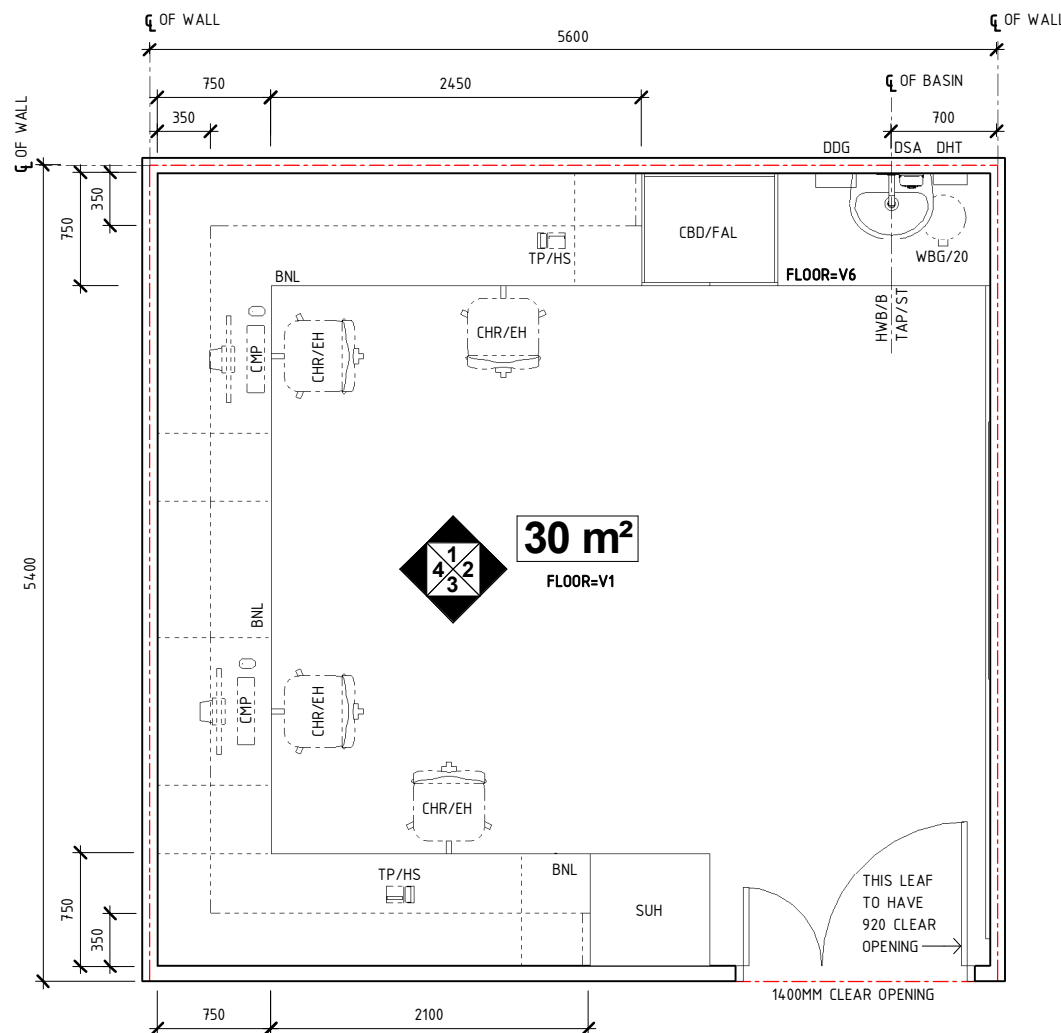
PLAN
