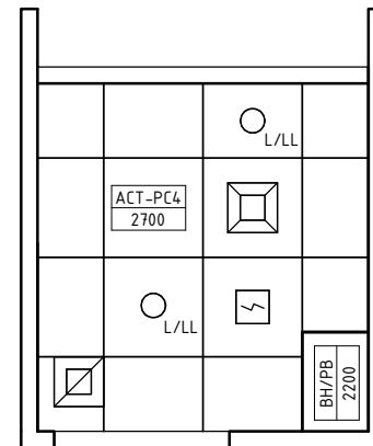
REFLECTED CEILING PLAN
