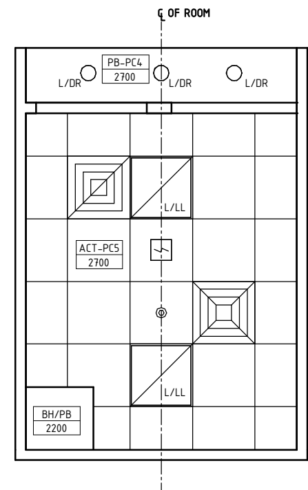
REFLECTED CEILING PLAN
