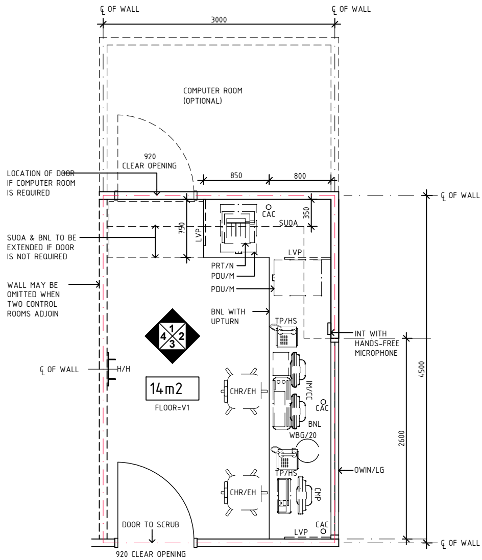
PLAN
