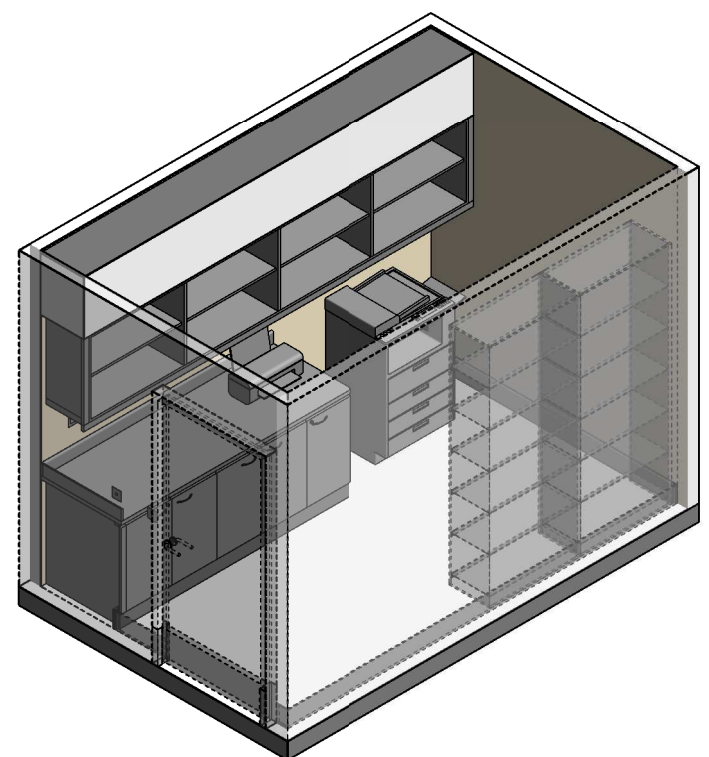
ISOMETRIC VIEW 2
