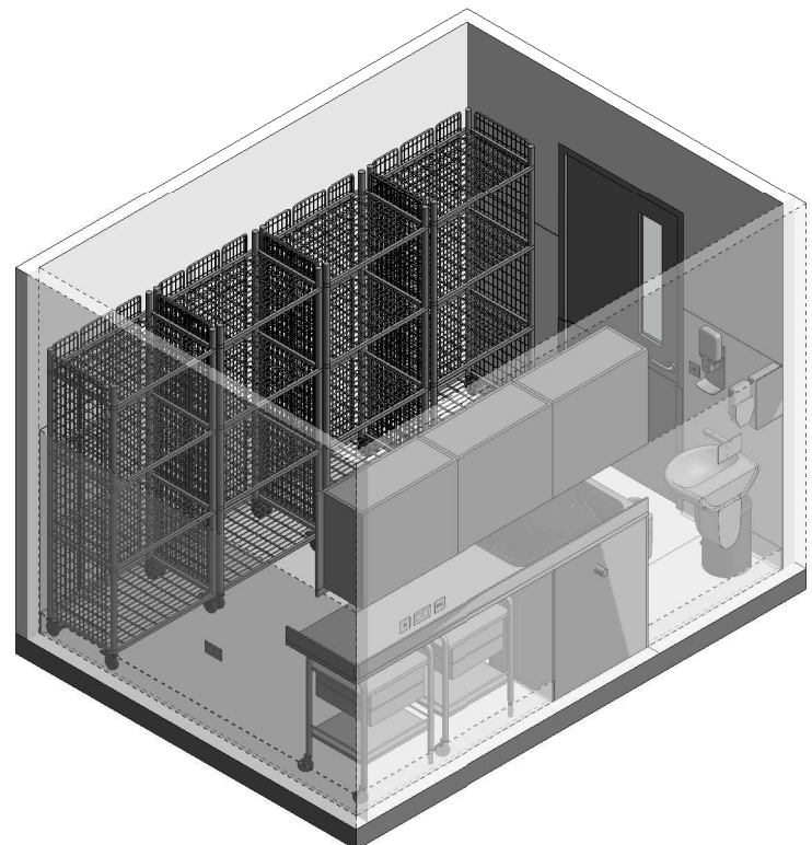
ISOMETRIC VIEW 02
