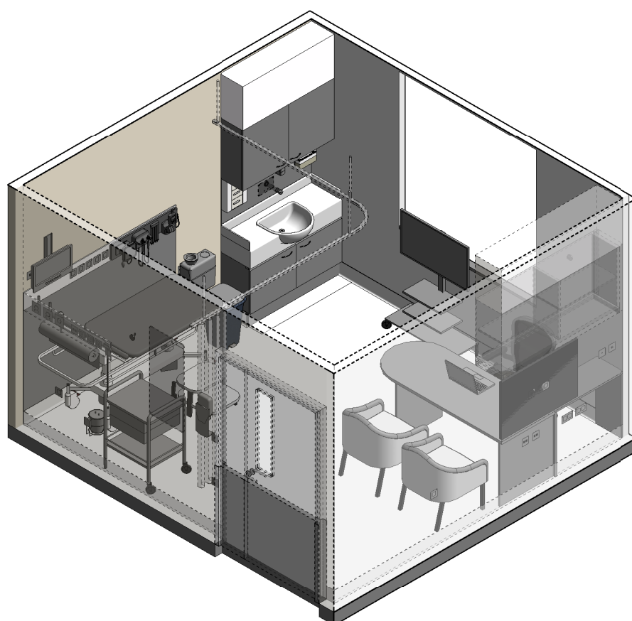
ISOMETRIC VIEW 01
