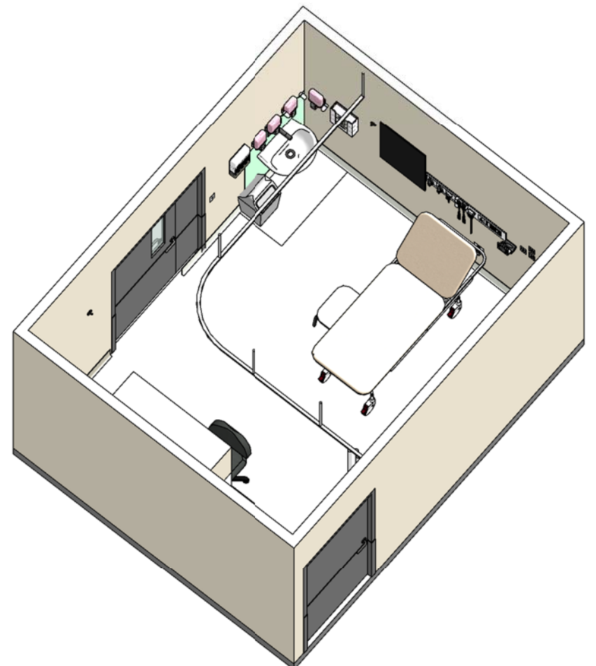
ISOMETRIC VIEW 01
