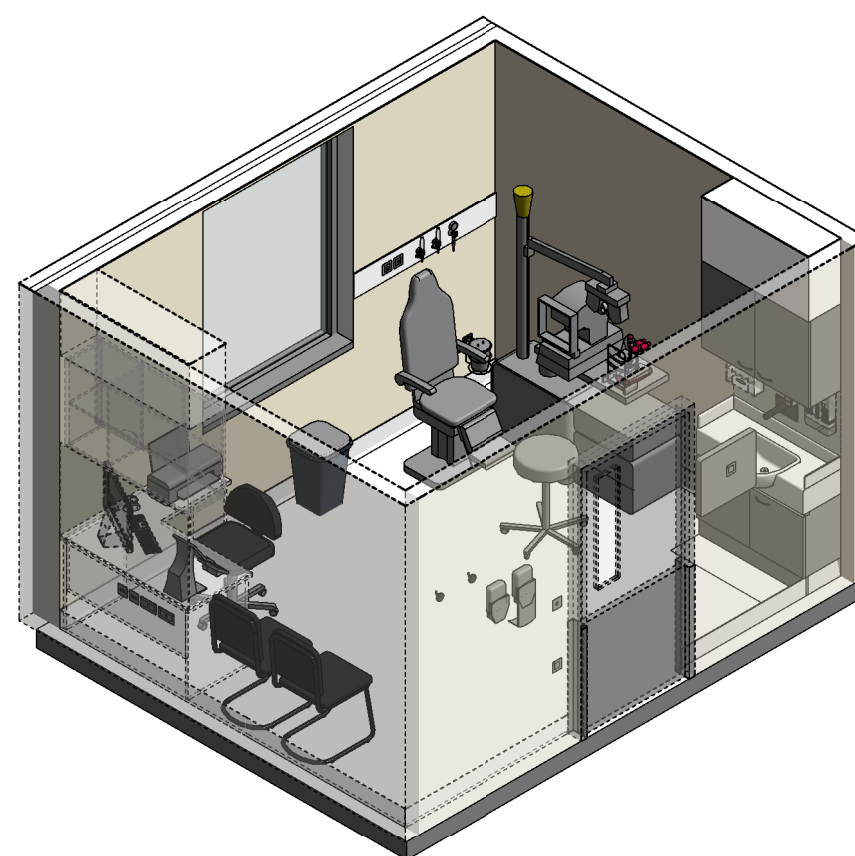
ISOMETRIC VIEW 02
