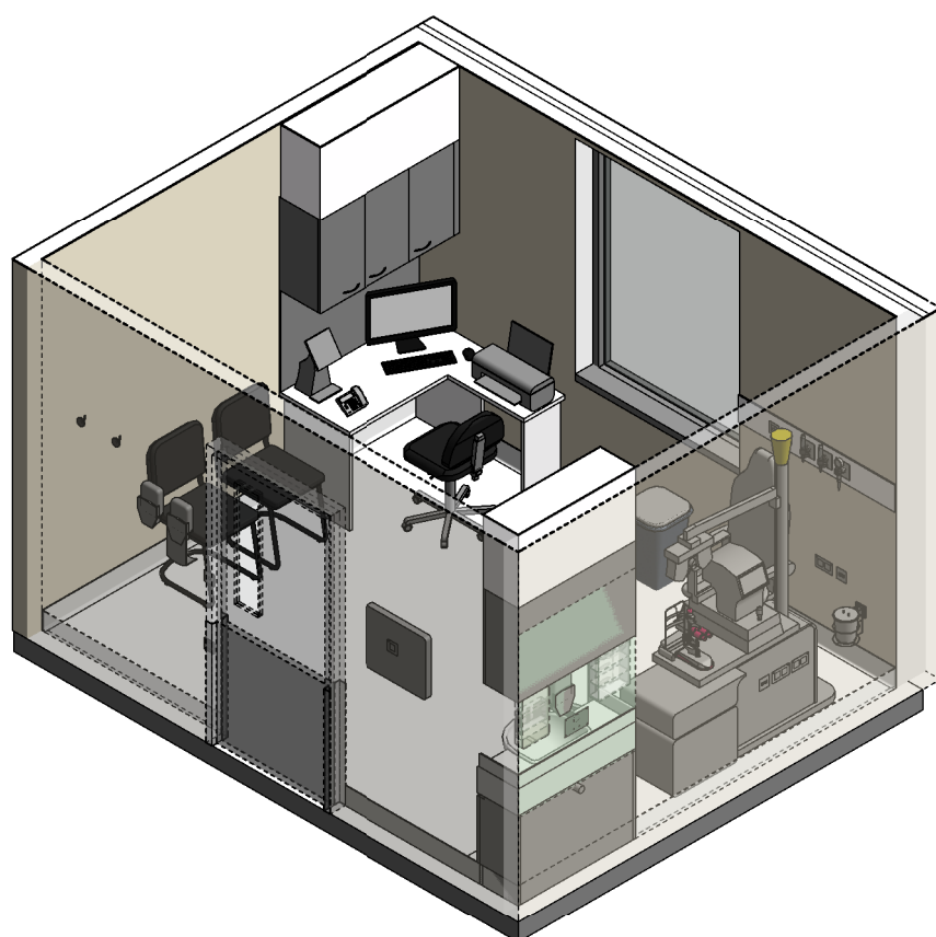
ISOMETRIC VIEW 1
