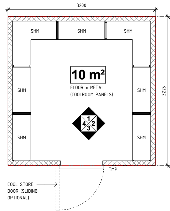
PLAN
