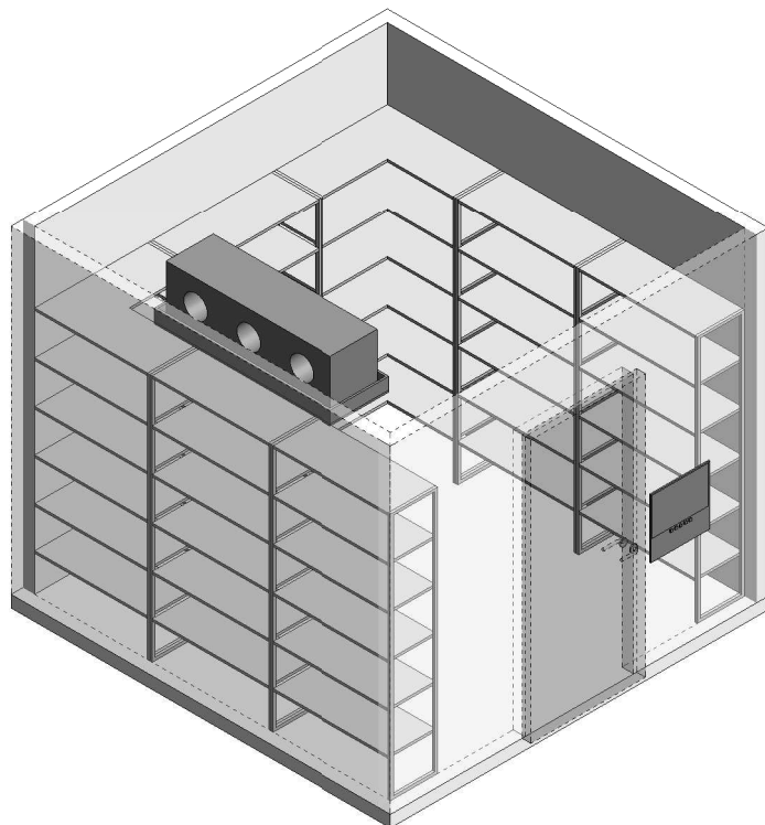
ISOMETRIC VIEW 1
