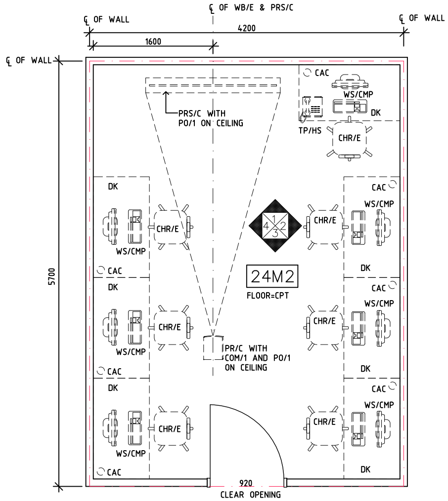
PLAN
