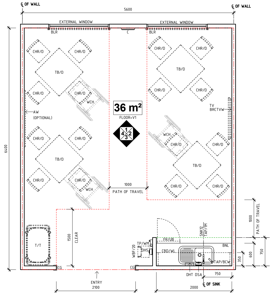
PLAN
