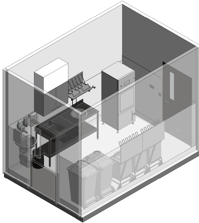
ISOMETRIC VIEW 01
