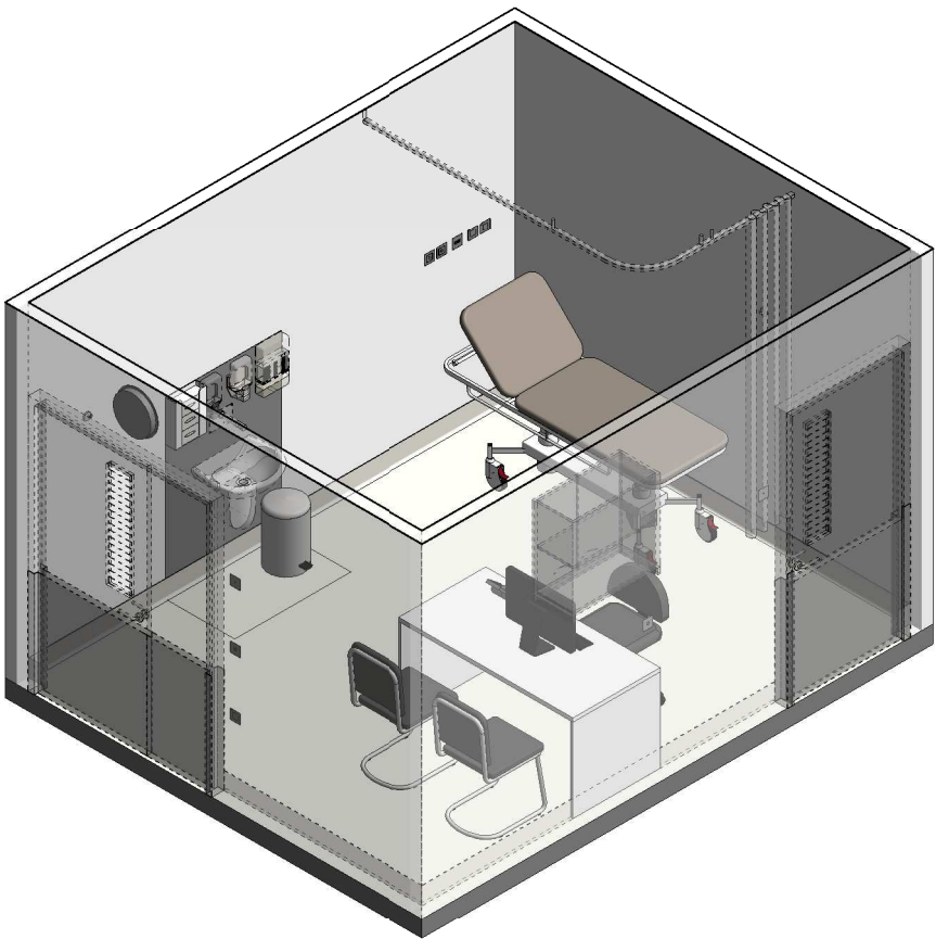
ISOMETRIC VIEW 01
