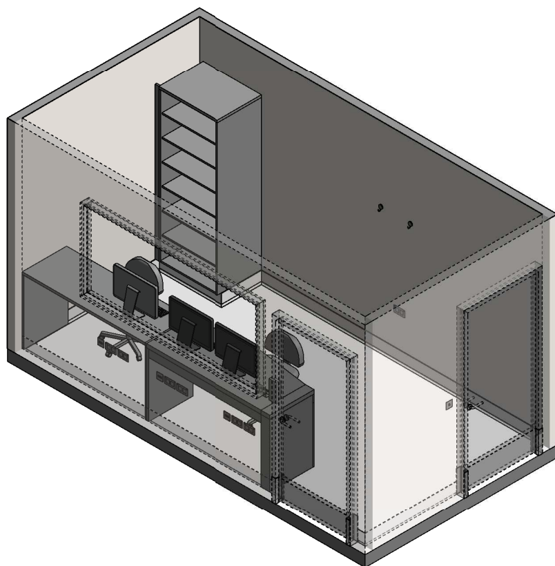
ISOMETRIC VIEW 01
