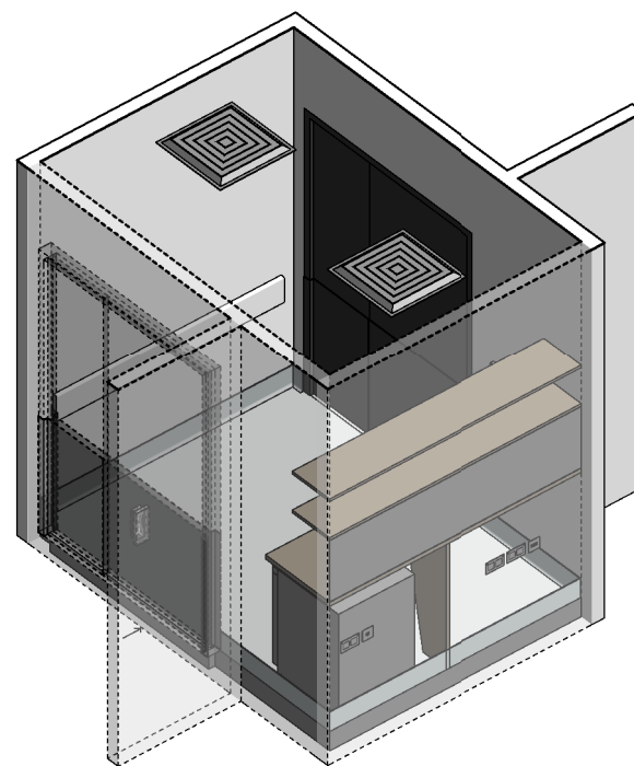
ISOMETRIC VIEW 02
