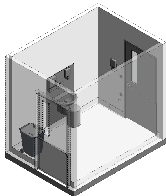
ISOMETRIC VIEW 02
