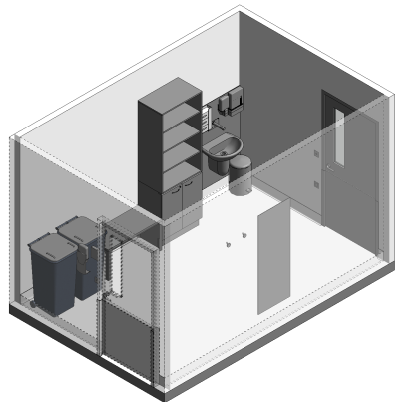
ISOMETRIC VIEW 02
