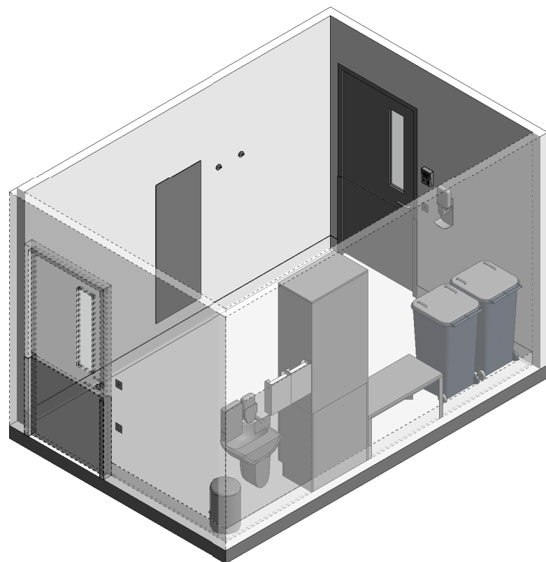
ISOMETRIC VIEW 01
