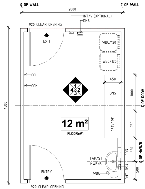
PLAN
