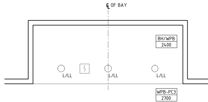
OPTION 1 REFLECTED CEILING PLAN
