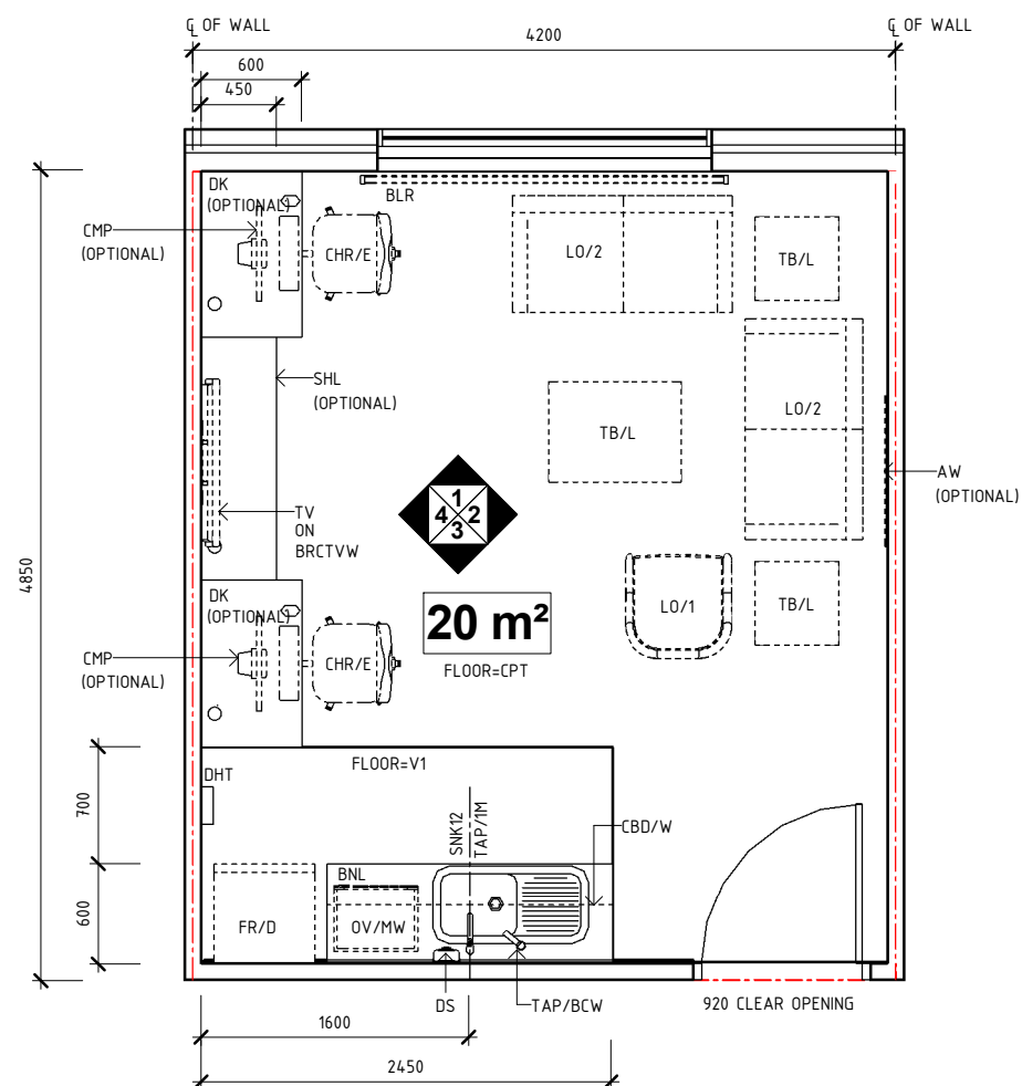
PLAN
