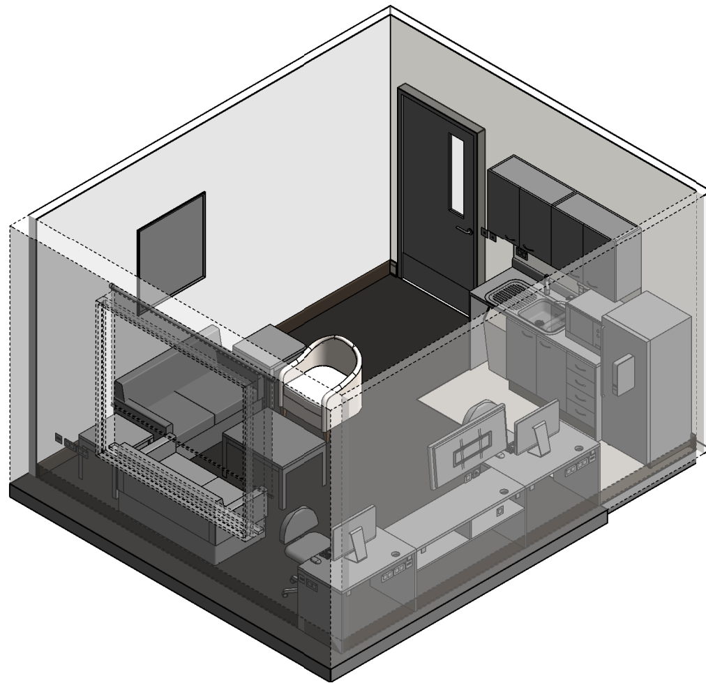
ISOMETRIC VIEW 01
