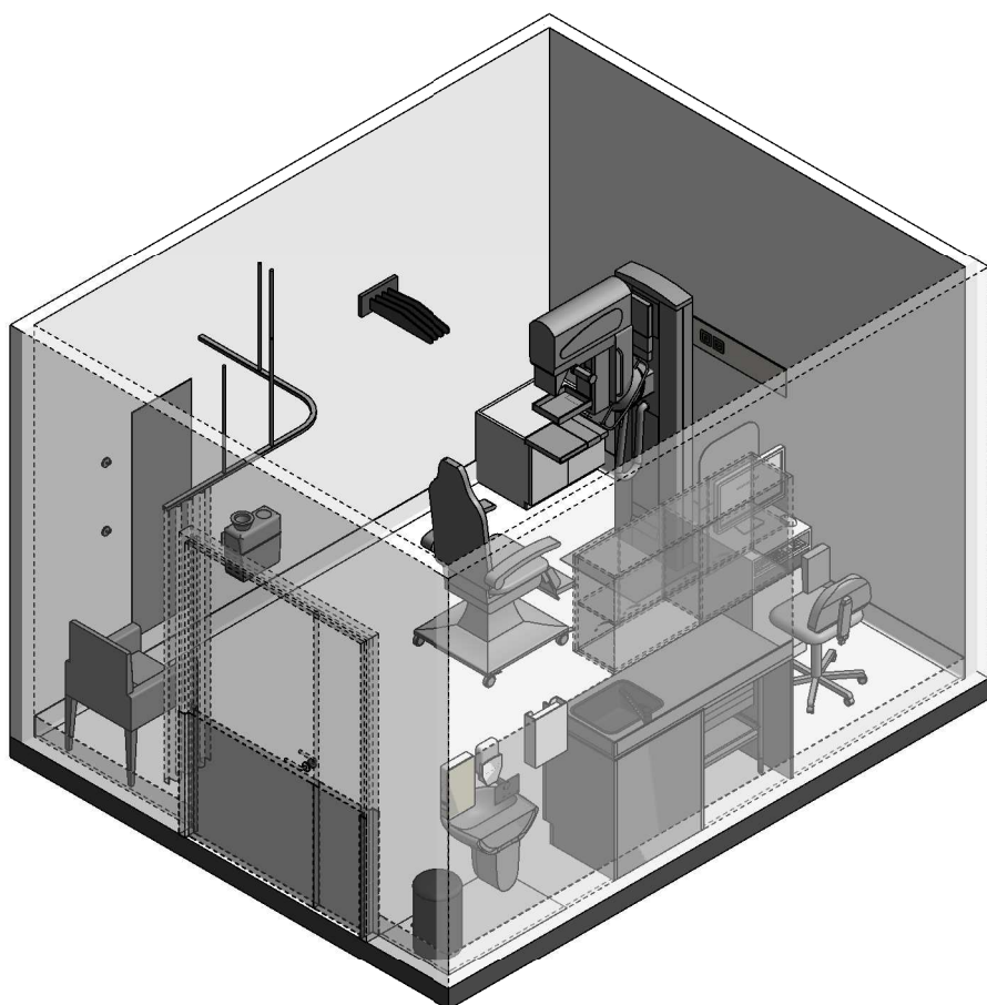
ISOMETRIC VIEW 01
