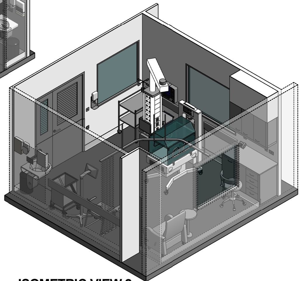
ISOMETRIC VIEW 2
