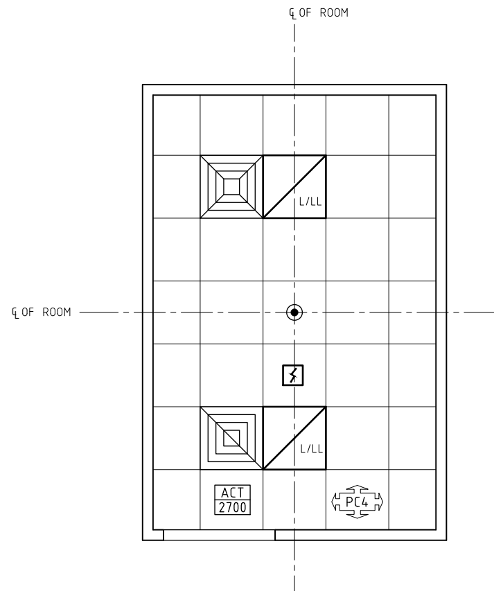
REFLECTED CEILING PLAN
