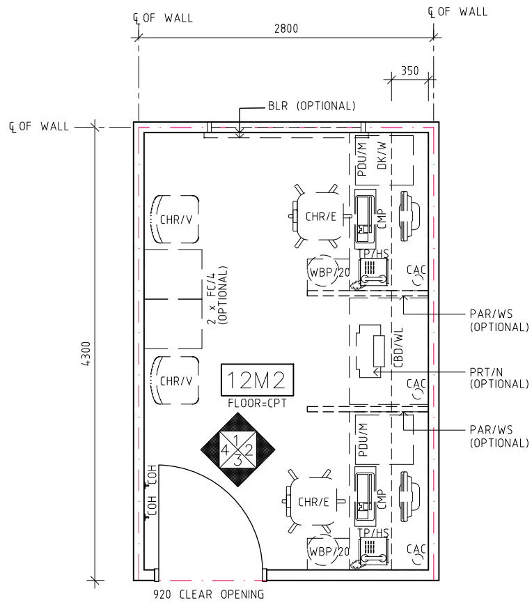
PLAN
