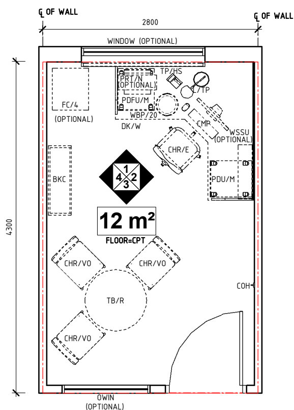
PLAN
