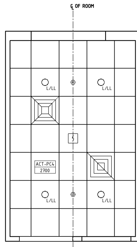
REFLECTED CEILING PLAN
