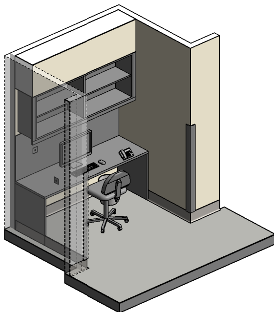
ISOMETRIC VIEW 01
