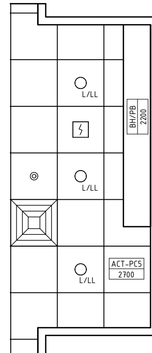
REFLECTED CEILING PLAN
