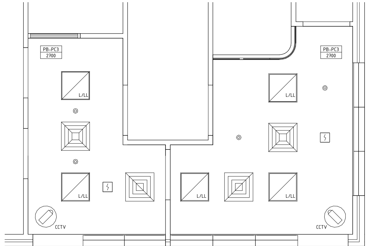
REFLECTED CEILING PLAN
